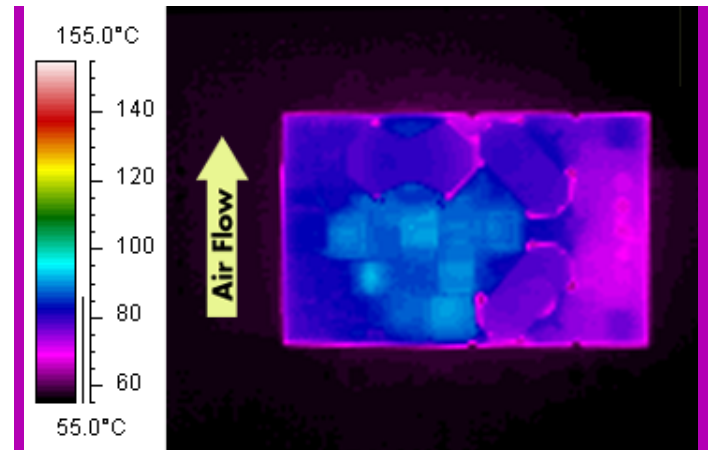
Figure 6: Thermal plot of converter at 9 amp load current with 55°C air flowing at the rate of 200 LFM. Air is flowing across the converter sideways from pin 3 to pin 1 (24V input).
