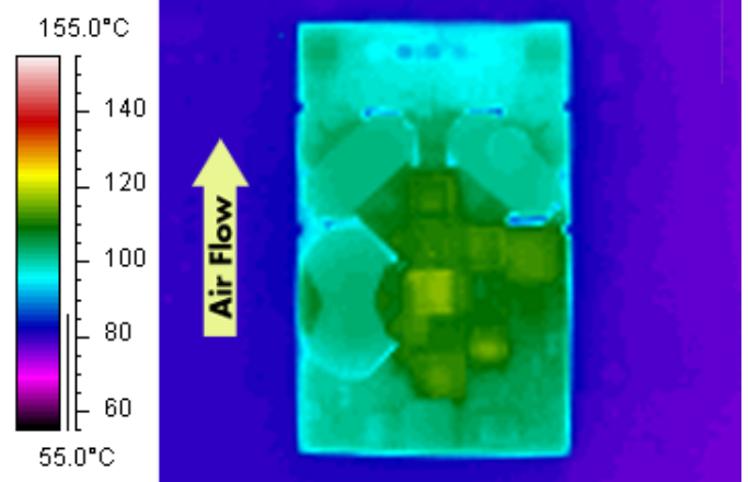
Figure 12: Thermal plot of converter at 8.7 amp load current with 85°C air flowing at the rate of 200 LFM. Air is flowing across the converter from input to output (48V input).
