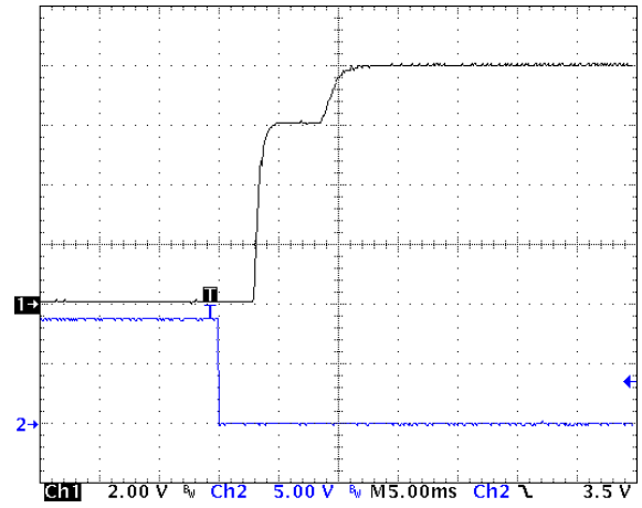
Figure 14: Turn-on transient at zero load (5 ms/div). Ch 1: V_{out} (2V/div). Ch 2: ON/OFF input (5V/div).
