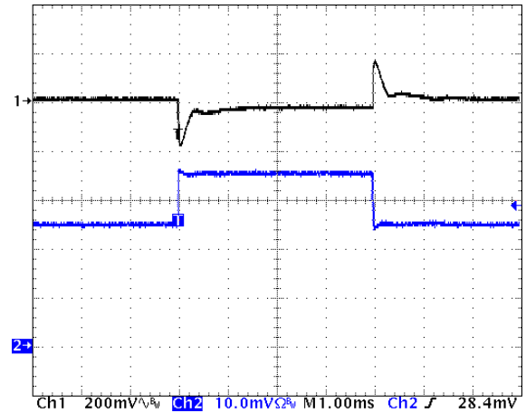
Figure 16: Output voltage response to step-change in load current (50%-75%-50% of I_{out(max)} ; di/dt = 5A/\mu s ). Load cap: 470\mu F , 30 mW ESR tantalum cap and 1\mu F ceramic cap. Ch 1: V_{out} (200mV/div), Ch 2: I_{out} (2A/div).
