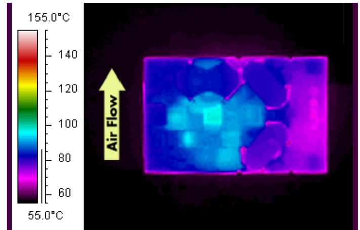
Figure 8: Thermal plot of converter at 9 amp load current with 55°C air flowing at the rate of 200 LFM. Air is flowing across the converter sideways from pin 3 to pin 1 (48V input).
