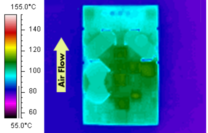
Figure 10: Thermal plot of converter at 9 amp load current with 85°C air flowing at the rate of 200 LFM. Air is flowing across the converter from input to output (24V input).
