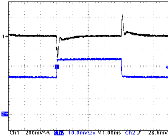
Figure 15: Output voltage response to step-change in load current (50%-75%-50% of I_{out(max)} ; di/dt = 0.1A/\mu s ). Load cap: 10\mu F , 100 mW ESR tantalum cap and 1\mu F ceramic cap. Ch 1: V_{out} (200mV/div), Ch 2: I_{out} (2A/div).
