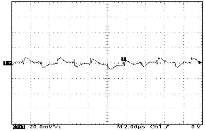
Figure 20: Output voltage ripple at nominal input voltage and rated load current (20 mV/div). Load capacitance: 1\ \mu\text{F} ceramic capacitor and 10\ \mu\text{F} tantalum capacitor. Bandwidth: 20 MHz. See Figure 17.
